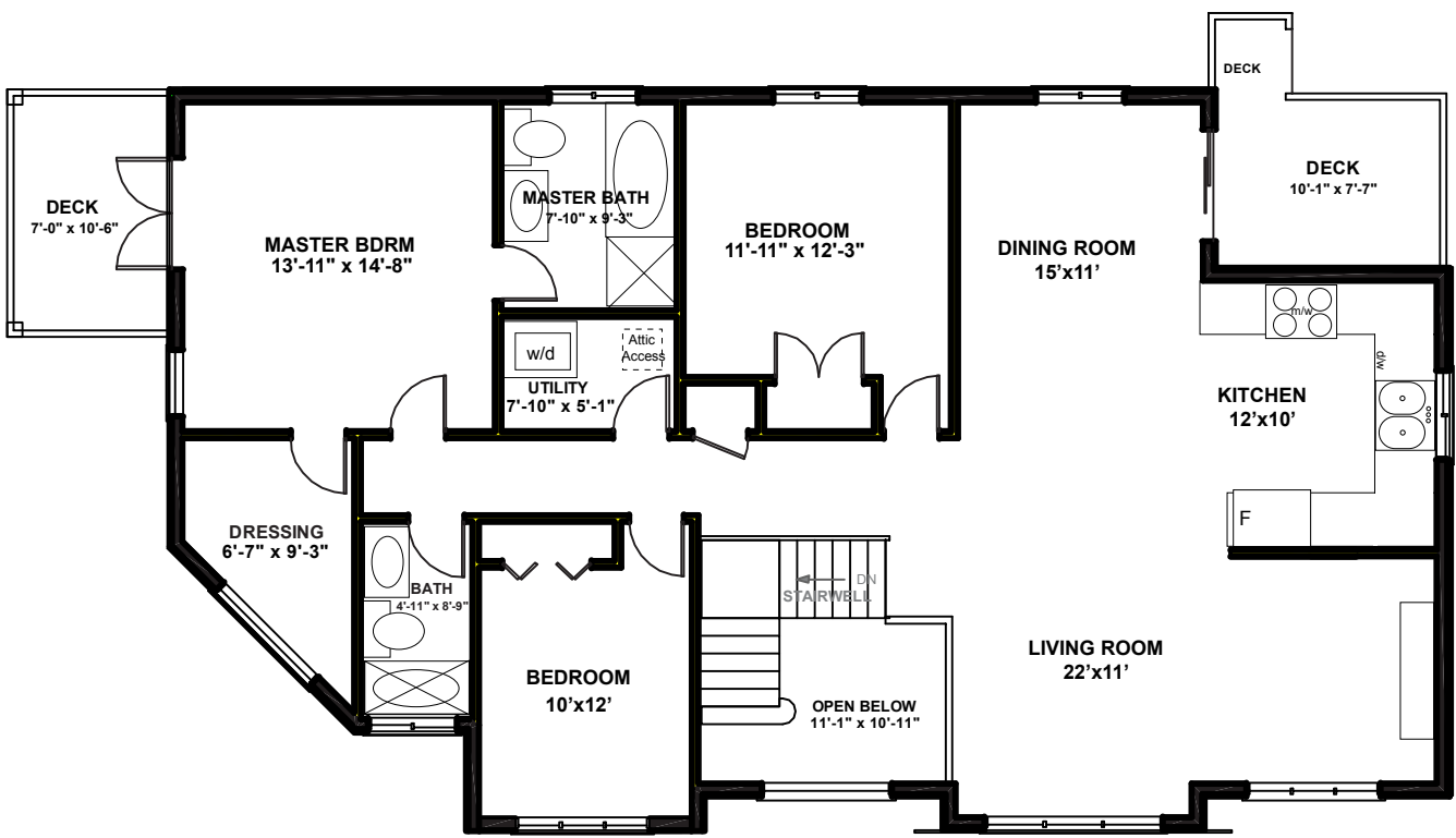
MAIN FLOOR PLAN 1554 sq ft
