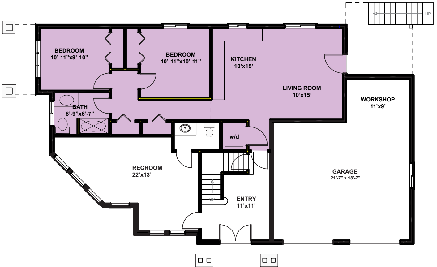
LOWER FLOOR PLAN 1275 sq ft
